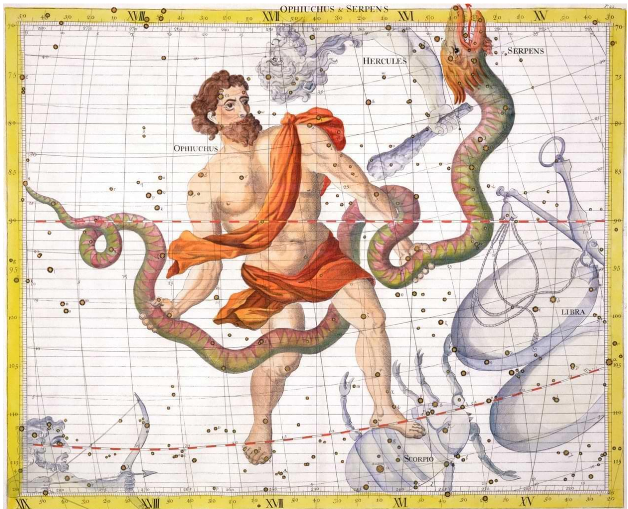
Ophiuchus/Apollo.
